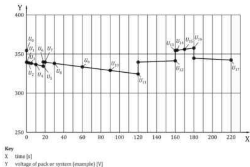
Figure 2: Pulse power characterization profile – Voltage
