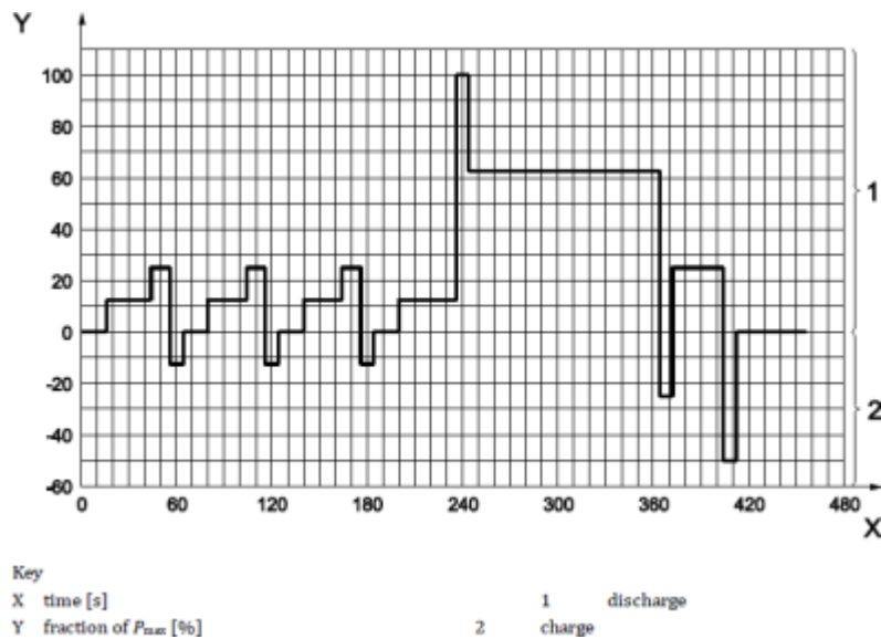
Figure 4: Profile for cycle life test – Dynamic discharge power
