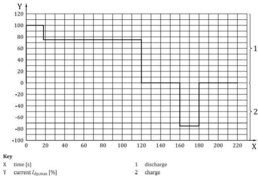
Figure 1: Pulse power characterization profile – current
