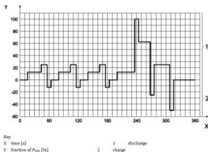
Figure 3: Profile for cycle life test – Dynamic discharge power profile A
